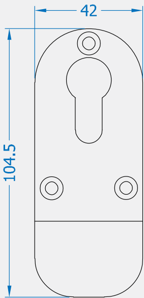
Front Profile
