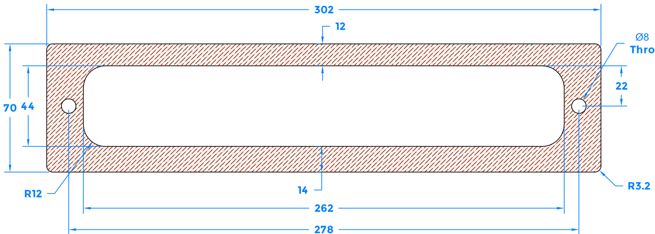
Recessed Fixing Routing Prep
