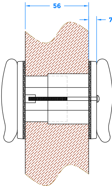
Surface Fixing
