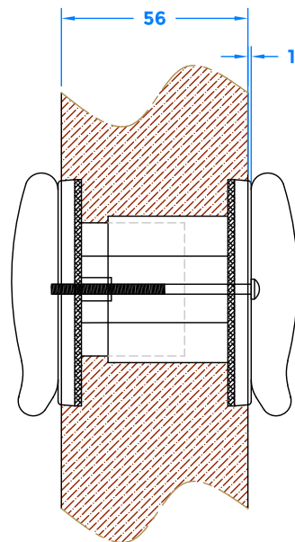
Recessed Fixing
