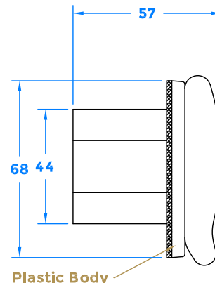
Internal
